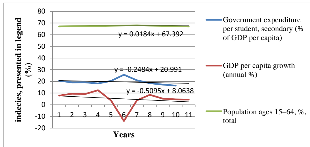
Fig. 3. The graphs of linear trends (specified in the legend of the graph) of three variables of a model according to the data of Lithuania (2004–2014)
