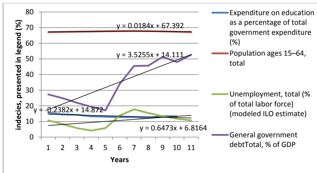
Fig. 2. The graphs of linear trends (specified in the legend of the graph ) of four variables of a model according to the data of Lithuania (2004–2014) 2
